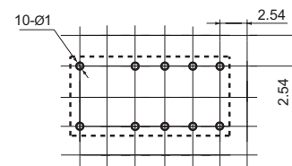
2 coils latching
