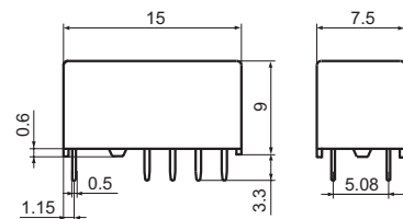
2 coils latching
