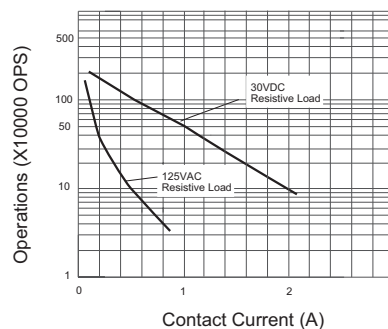
LIFE CURVE
